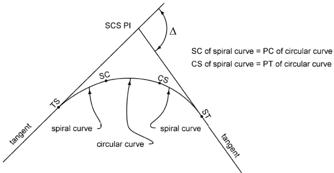
Figure 1: Placement of spiral curve.
